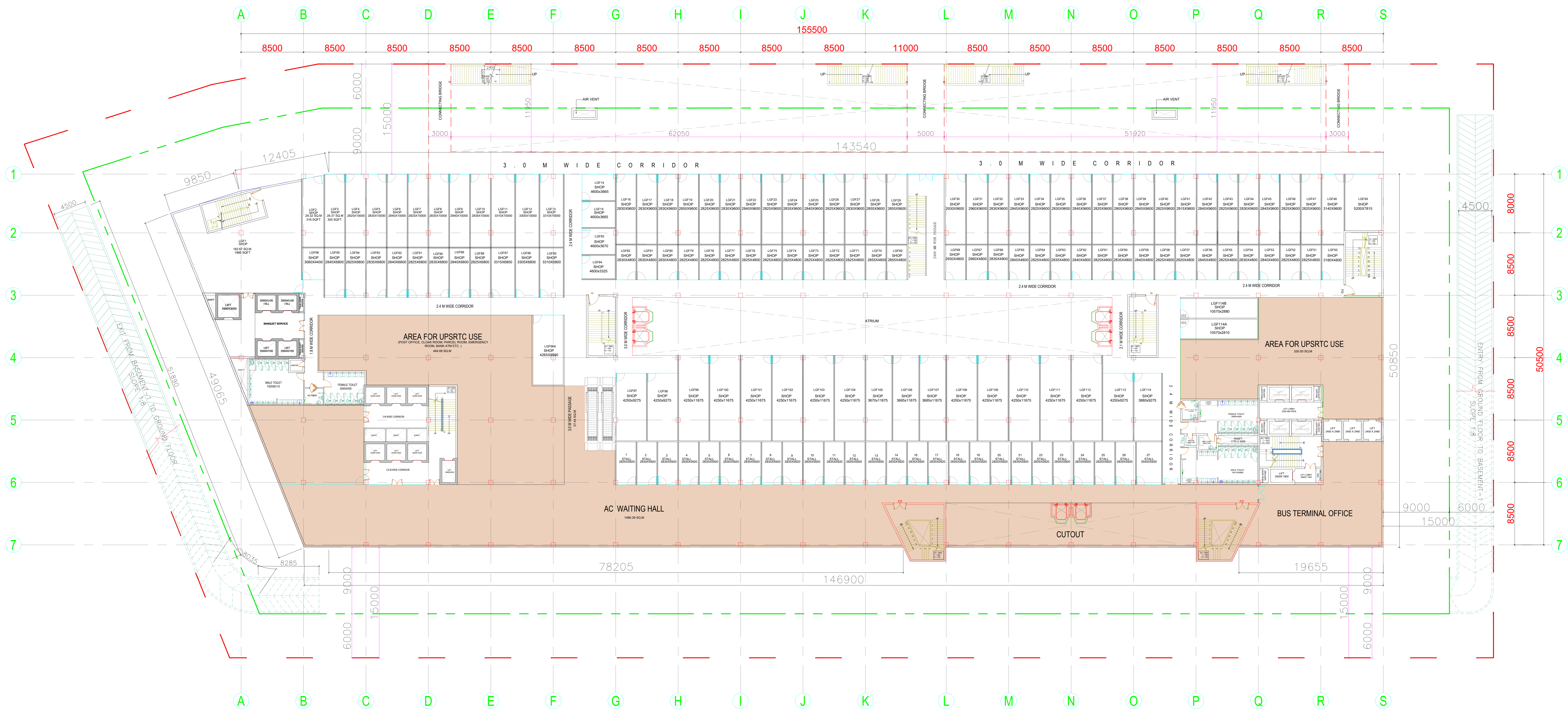
LOWER GROUND FLOOR PLAN
